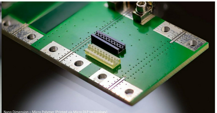
Nano Dimension – Micro Polymer (Printed via Micro DLP technology)
