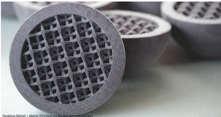
Desktop Metal – Metal (Printed via Binder-Jet technology)
