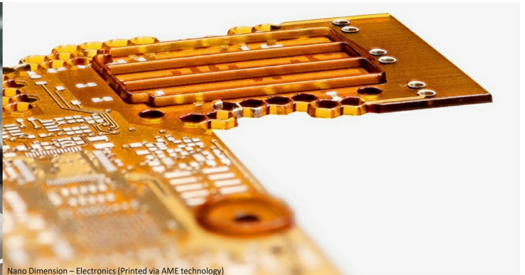
Nano Dimension – Electronics (Printed via AME technology)
