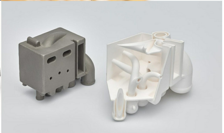
Nano Dimension – Ceramics (Printed via Foil DLP technology)
